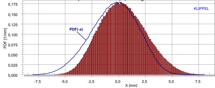
Displacement PDF (X) Histogram
